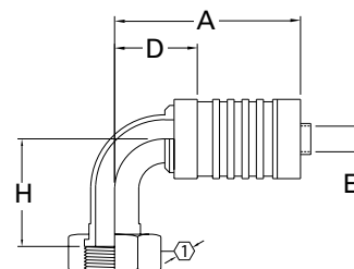
ORS Swivel 90° Elbow (long) FJ9721
