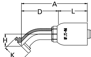
45° Elbow Split Flange Code 61
