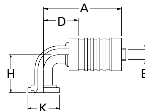
90° Elbow Split Flange FC5329 Code 62
