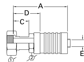
ORS Swivel Straight FJ9718
