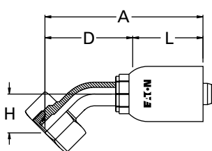
DKOS Swivel 45° Elbow
