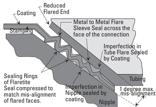
Flaretite Seal Joint Section of Applied Seal
