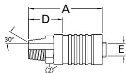
Male Pipe FC5258
